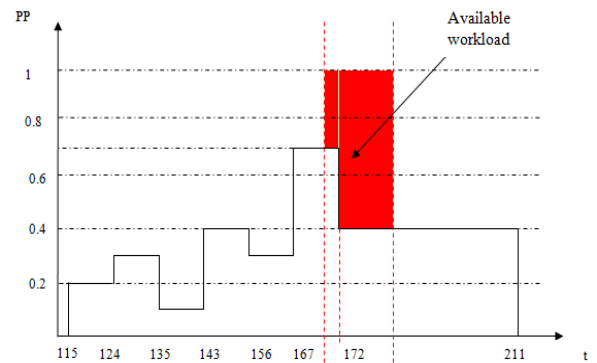
Fig. 3b: Step 2, computing available workload
