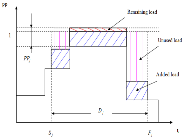
Fig 6: A task rejected using the traditional approach
