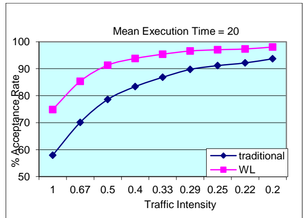
Fig 10: Acceptance rate at mean execution time ( 1/\mu ) = 20 and different traffic intensity
