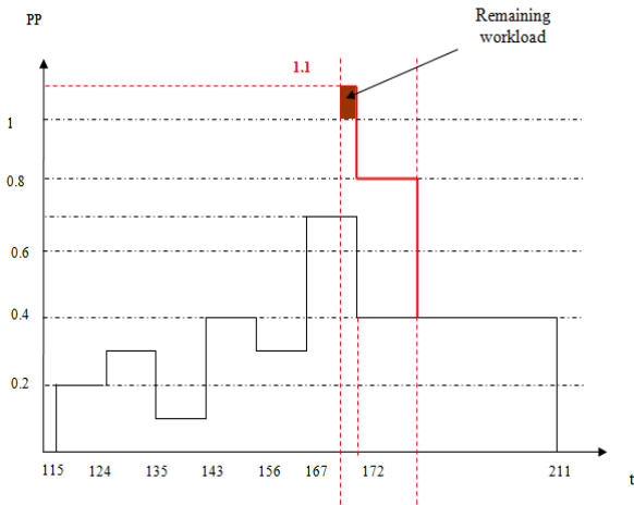
Fig. 3c: Step 3, computing remaining workload
