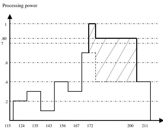
Fig. 4: RG after accepting T_5
